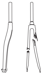
Figure 2.5: Left: Metal fork bent when overloaded. Right: Carbon fork withstood a higher load, but completely separated when overloaded.
